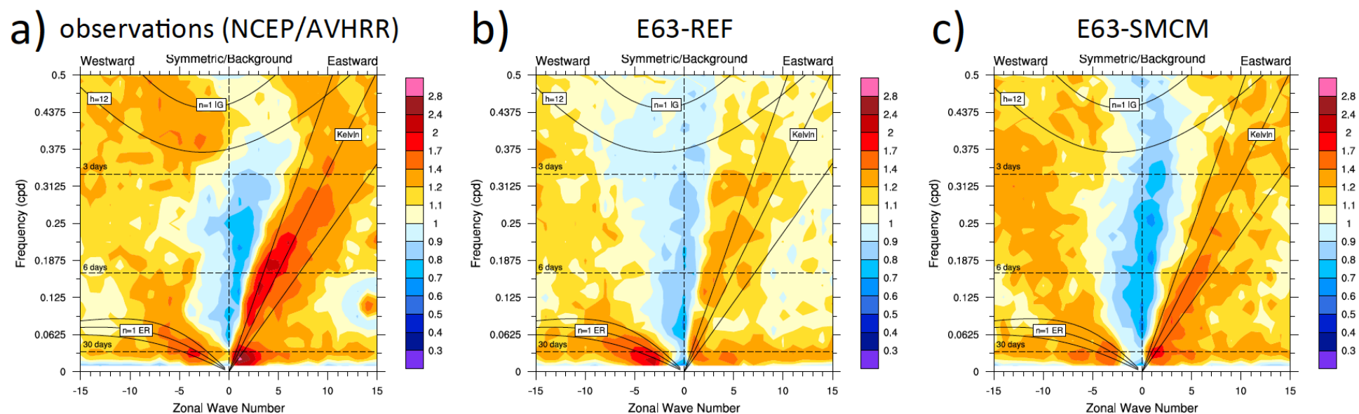
Frequency-wavenumber spectra of OLR
