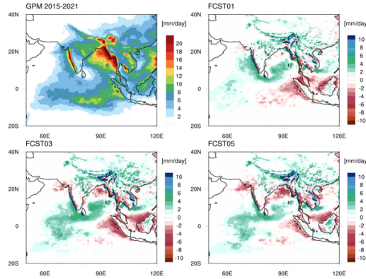
Figure 1: Mean state and biases (c-d) computed w.r.t GPM rainfall observations during monsoon. One disparity is the presence of very high MSE ( 60 \text{ W/m}^2 \sim 3 \text{ mm/day} ) seen in the model layers between surface to 925 hPa. Horizontal advection of MSE indicates dryness prior to the peak break conditions over CI. The surface fluxes and net radiation are in phase with MSE, and the contribution of surface turbulent fluxes are relatively minimal compared to other MSE terms. Preliminary results are encouraging and indicating the advantage of using PODs as one of the verification tools for assessing model forecasts.
