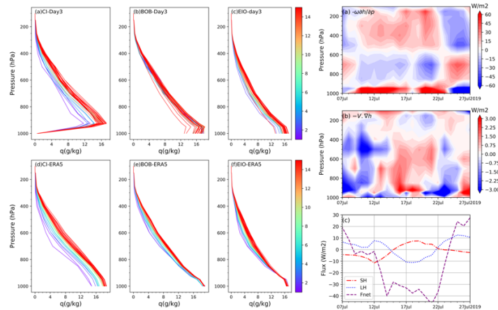
Figure 2: Left panel: Conditionally averaged specific humidity and rainfall over three selected regions. Right panel: MSE budget terms for a strong individual break event in 2019 over central India.
