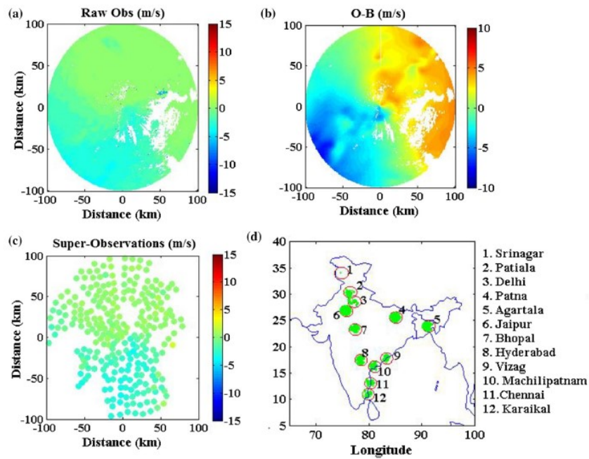
Fig 1: a) Raw DWR observation; b) observed minus background (O – B); c) super-observations from the Chennai DWR station (as an example on 00 UTC 26 July 2016).
