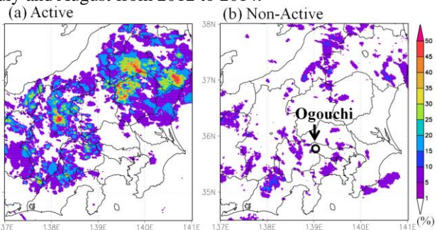
Figure 2. Horizontal distributions of occurrence frequency of rainfall greater than 1 mm h^{-1} at 17 JST for (a) active and (b) non-active cases.
