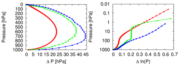
Fig. 1: Vertical layer placement. An example of GSM L100 created by the procedure described in the text (red), GSM L60 in operation (green), and GSM L40 which was in operation until 2007. Profiles of \Delta p_{k-1/2} (left) and \Delta \log(p_{k-1/2}) (right). Note that \Delta \log(p_{k-1/2}) at the top is infinity.
