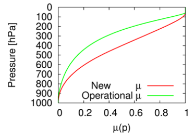
Fig. 2: Profile of \mu(p) (a weight of coefficient of A in the pressure p for layers, where p_s = 1000 hPa is assumed). The new function (red) and the function used in the operational model (green).
